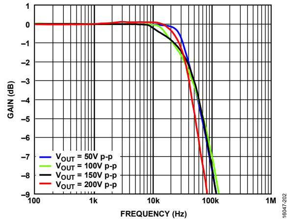
Figure 22. Large Signal Frequency Response at Various Output Swings with Input Clamping Diodes (See the Slew Boost Circuit and Protection Section), T_A = 25^\circ\text{C} , A_V = 40 , V_S = \pm 110\text{ V} , R_F = 100\text{ k}\Omega , R_{LOAD} = 10\text{ k}\Omega , R_{ADJ} = 0\ \Omega
