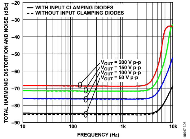
Figure 38. Total Harmonic Distortion and Noise vs. Frequency at Various Large Output Swings, T_A = 25^\circ\text{C} , A_V = 20 , V_S = \pm 110 \text{ V} , R_F = 100 \text{ k}\Omega , R_{LOAD} = 10 \text{ k}\Omega , R_{ADJ} = 0 \Omega
