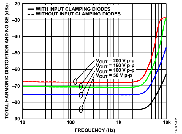
Figure 39. Total Harmonic Distortion and Noise vs. Frequency at Various Large Output Swings, T_A = 25^\circ\text{C} , A_V = 40 , V_S = \pm 110 \text{ V} , R_F = 100 \text{ k}\Omega , R_{LOAD} = 10 \text{ k}\Omega , R_{ADJ} = 0 \Omega
