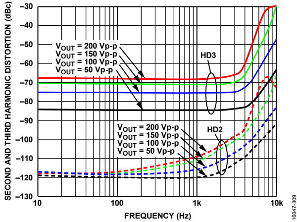
Figure 41. Second Harmonic Distortion (HD2) and Third Harmonic Distortion (HD3) vs. Frequency at Various Output Swings, T_A = 25^\circ\text{C} , A_V = 40 , V_S = \pm 110\text{V} , R_F = 100\text{ k}\Omega , R_{LOAD} = 10\text{ k}\Omega , R_{ADJ} = 0\ \Omega
