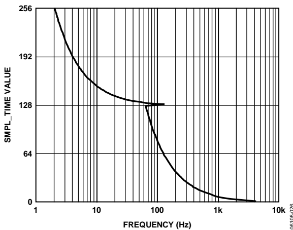
Figure 29. SMPL_TIME Values vs. Sample Frequency
