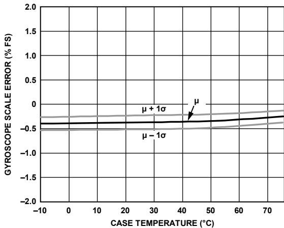
Figure 10. Gyroscope Scale (Sensitivity) Error vs. Case Temperature
