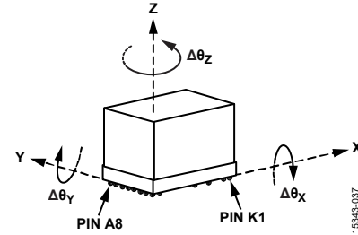
Figure 36. Delta Angle Axis and Polarity Assignments
