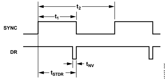
Figure 5. Input Clock Timing Diagram, Direct Sync Mode, Register MSC_CTRL, Bits[4:2] = 001 (Binary)
