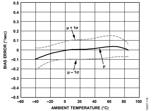
Figure 16. ADIS16477-2 Gyroscope Bias Error vs. Ambient Temperature
