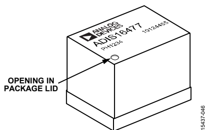
Figure 50. Pressure Relief Hole
