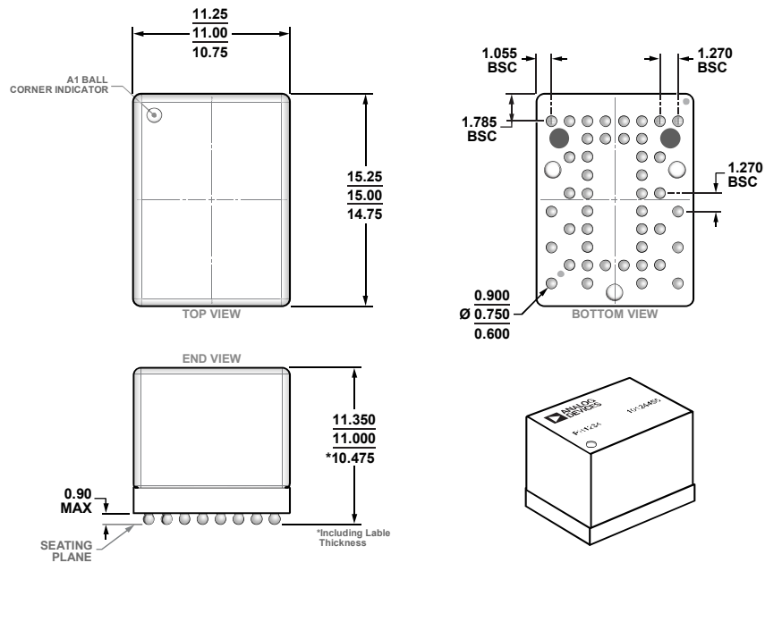
Figure 55. 44-Ball Ball Grid Array Module [BGA] (ML-44-1) Dimensions shown in millimeters
