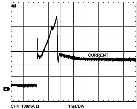
Figure 39. Transient Current Demand, Peak Demand
