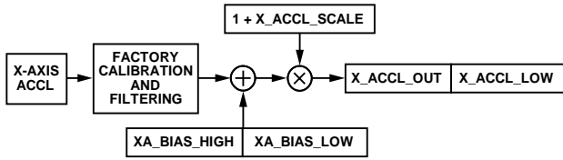
Figure 47. User Calibration Signal Path, Accelerometers
