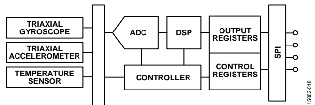
Figure 22. Basic Operation
