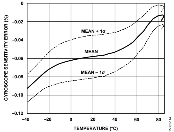
Figure 14. Gyroscope Sensitivity Error vs. Temperature, Hot to Cold, ADIS16495-1
