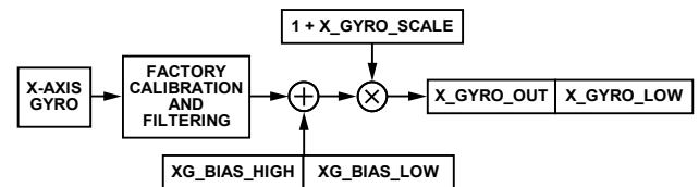
Figure 45. User Bias/Scale Adjustment Registers in Gyroscope Signal Path
