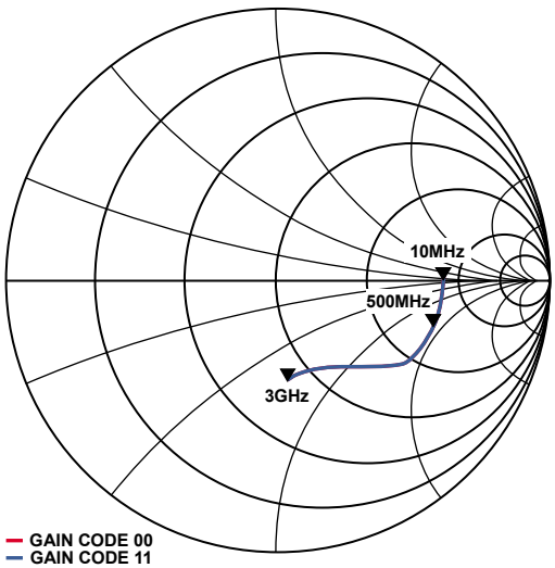
Figure 37. S11 (re: 50 Ω) vs. Frequency over V_{GAIN} for VGA1
