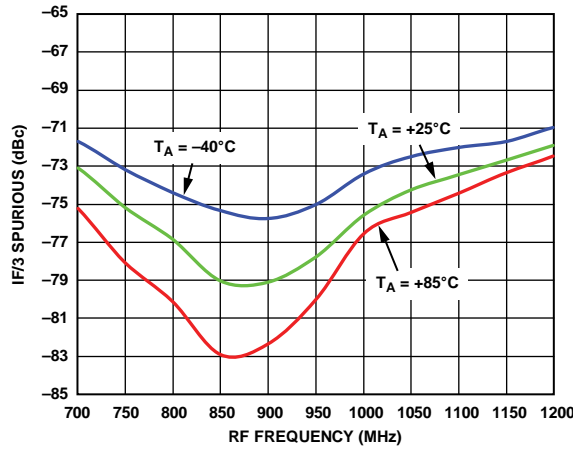
Figure 26. IF/3 Spurious vs. RF Frequency
