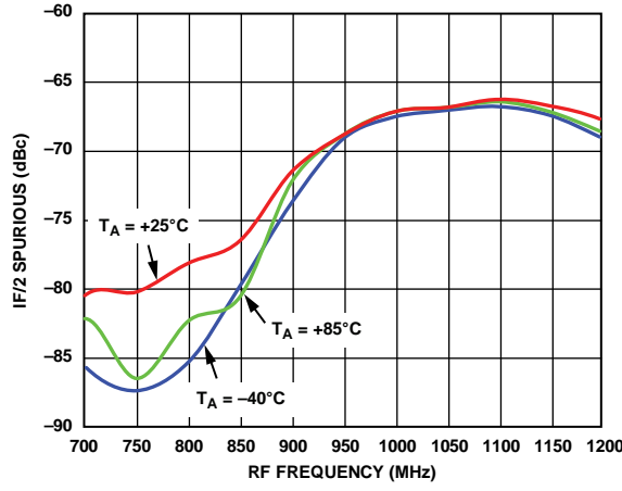
Figure 25. IF/2 Spurious vs. RF Frequency
