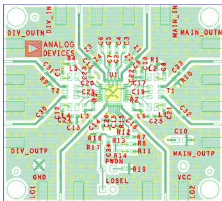
Figure 55. Evaluation Board Top Layer
