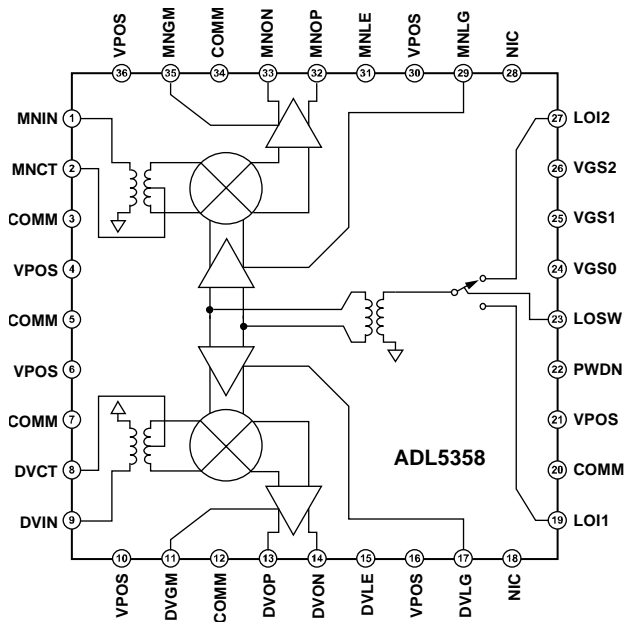
Figure 52. Simplified Schematic
