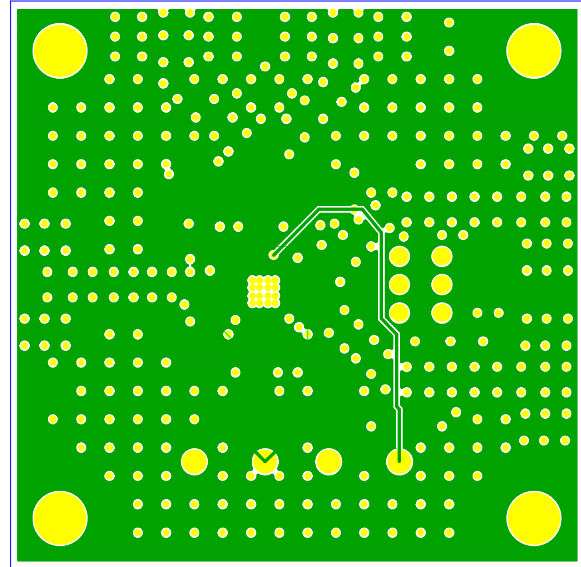
Figure 52. Evaluation Board Power Plane, Internal Layer 2
