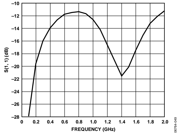
Figure 53. Differential RF Port Return Loss
