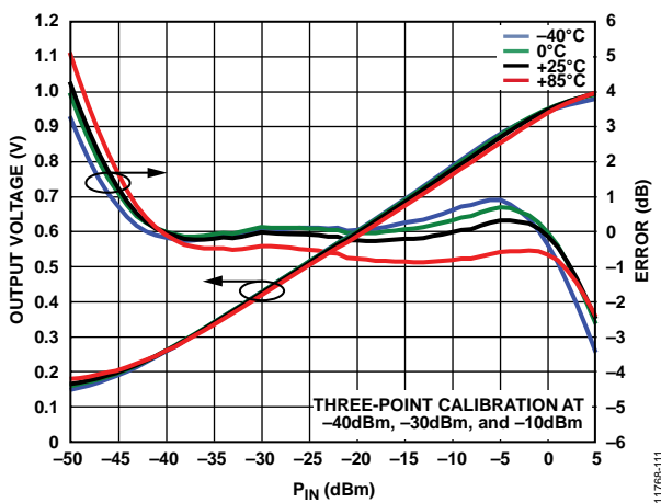
Figure 11. V_{LOG} and Log Conformance Error vs. P_{IN} over Temperature at 100 MHz
