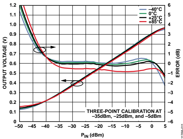
Figure 10. V_{LOG} and Log Conformance Error vs. P_{IN} over Temperature at 50 MHz
