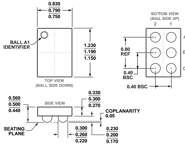
Figure 53. 6-Ball Wafer Level Chip Scale Package [WLCSP] (CB-6-14) Dimensions shown in millimeters
