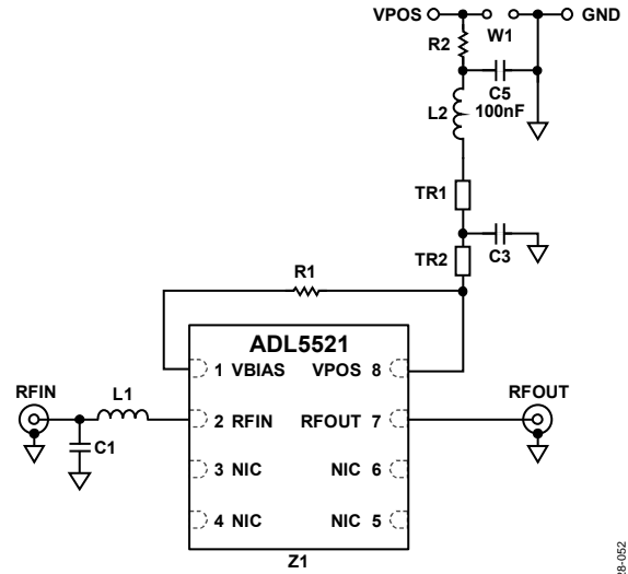
NIC = NO INTERNAL CONNECTION. DO NOT CONNECT TO THIS PIN. 06828-052
