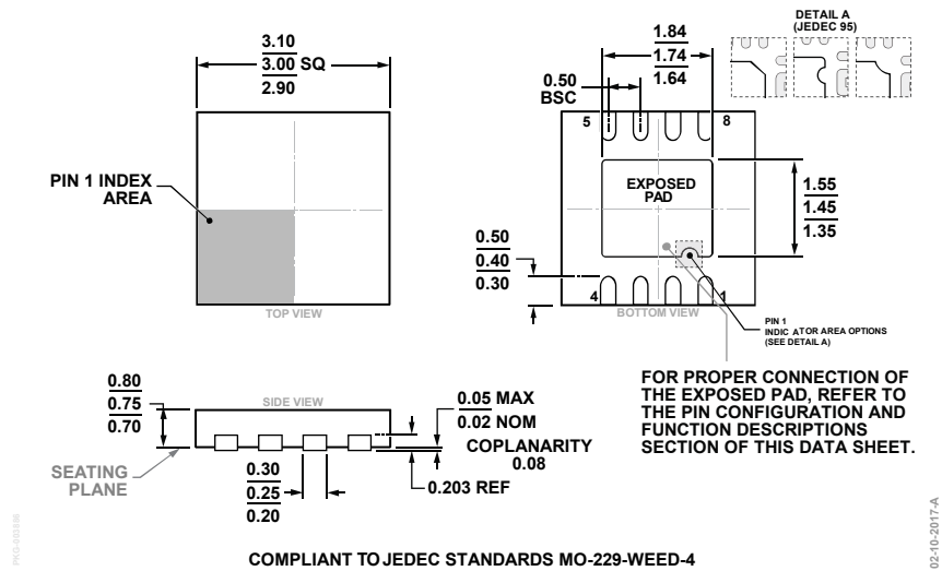
COMPLIANT TO JEDEC STANDARDS MO-229-WEED-4 Figure 65. 8-Lead Lead Frame Chip Scale Package [LFCSP] 3 mm x 3 mm Body and 0.75 mm Package Height (CP-8-13) Dimensions shown in millimeters
