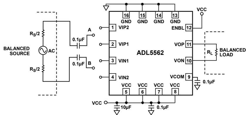
Figure 33. Basic Connections
