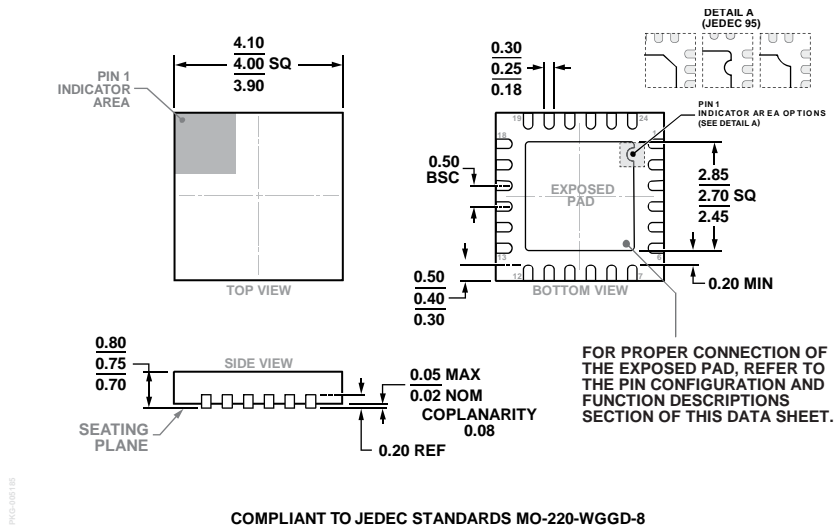
COMPLIANT TO JEDEC STANDARDS MO-220-WGGD-8 Figure 113. 24-Lead Lead Frame Chip Scale Package [LFCSP] 4 mm × 4 mm Body and 0.75 mm Package Height (CP-24-8) Dimensions shown in millimeters
