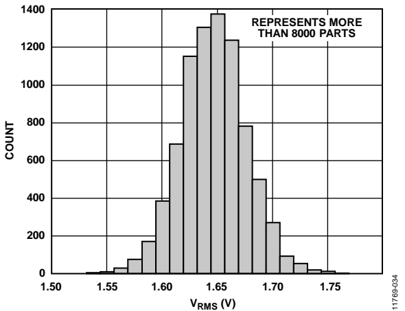
Figure 29. Distribution of V_{RMS} , P_{IN} = 8 dBm, 900 MHz
