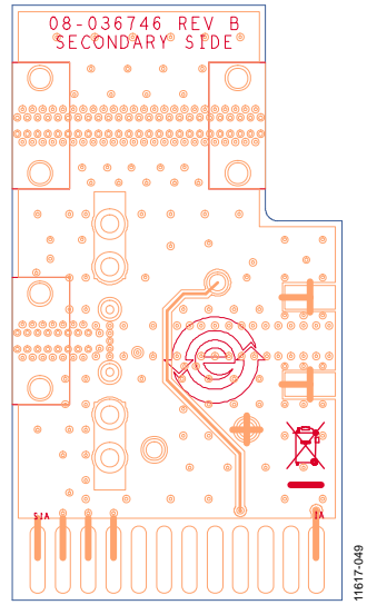
Figure 49. ADL6010 Evaluation Board Layout, Bottom Side
