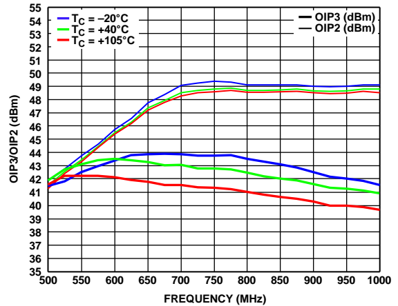
Figure 16. OIP3/OIP2 vs. Frequency for Various Temperatures
