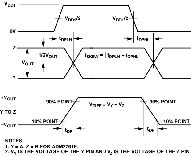
Figure 3. Driver Propagation Delay, Rise and Fall Timing
