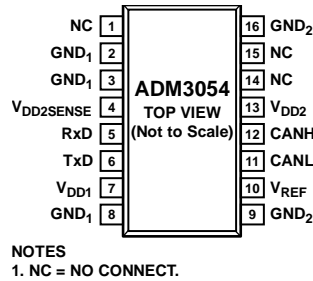
Figure 2. Pin Configuration
