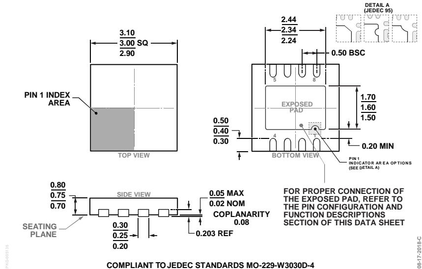
COMPLIANT TO JEDEC STANDARDS MO-229-W3030D-4 Figure 71. 8-Lead Lead Frame Chip Scale Package [LFCSP] 3 mm x 3 mm Body and 0.75 mm Package Height (CP-8-11) Dimensions shown in millimeters
