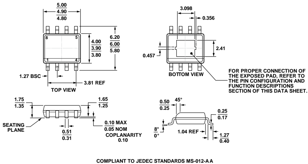
COMPLIANT TO JEDEC STANDARDS MS-012-A A Figure 72. 8-Lead Standard Small Outline Package, with Exposed Pad [SOIC_N_EP] Narrow Body (RD-8-2) Dimensions shown in millimeters
