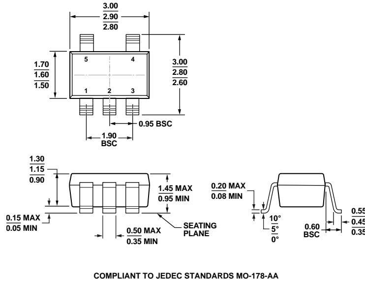
COMPLIANT TO JEDEC STANDARDS MO-178-AA Figure 26. 5-Lead Small Outline Transistor Package [SOT-23] (RJ-5)
