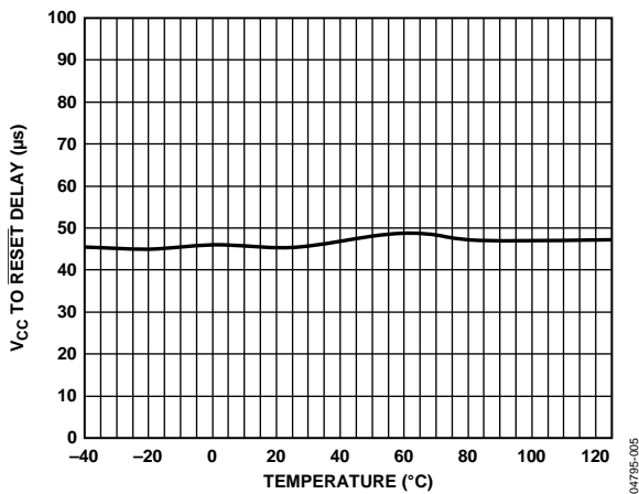
Figure 5. V_{CC} to \overline{\text{RESET}} Output Delay vs. Temperature
