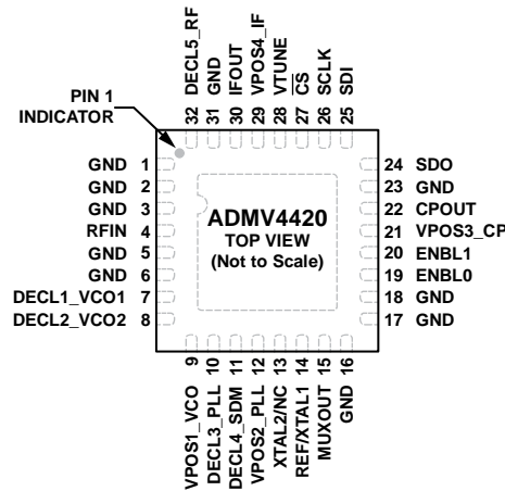
Figure 3. Pin Configuration
