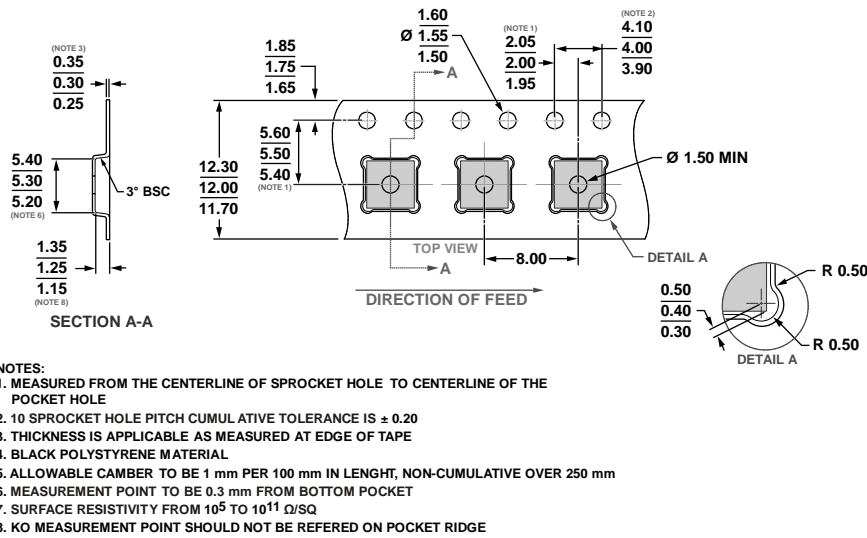
Figure 134. 32-Lead Lead Frame Chip Scale Package [LFCS] Tape and Reel Outline Dimensions Dimensions shown in millimeters
