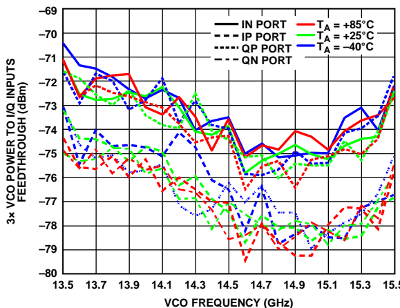
Figure 68. 3x VCO to I/Q Inputs Feedthrough vs. VCO Frequency over Temperature, Uncalibrated
