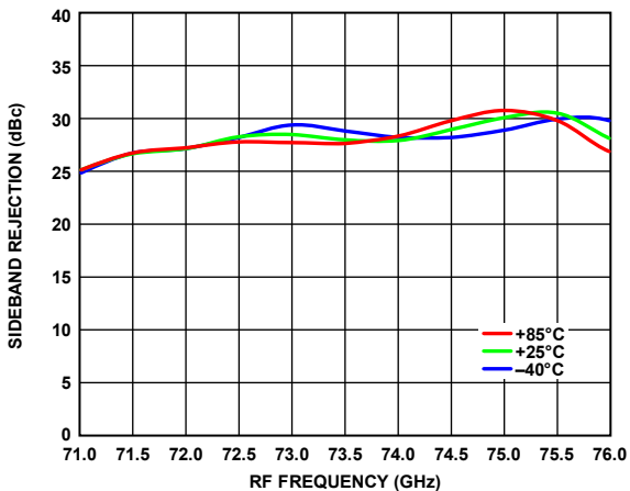
Figure 38. Sideband Rejection vs. RF Frequency over Temperature, Gain = 23.5\text{ dB}
