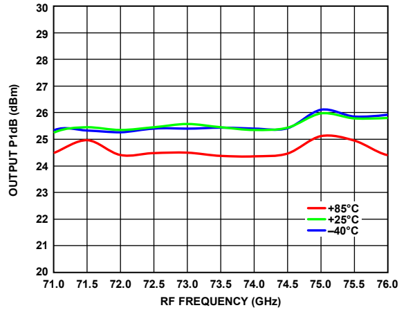
Figure 40. Output P1dB vs. RF Frequency over Temperature, Gain = 23.5\text{ dB}
