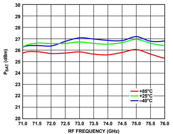
Figure 41. P_{SAT} vs. RF Frequency over Temperature, Gain = 23.5\text{ dB}
