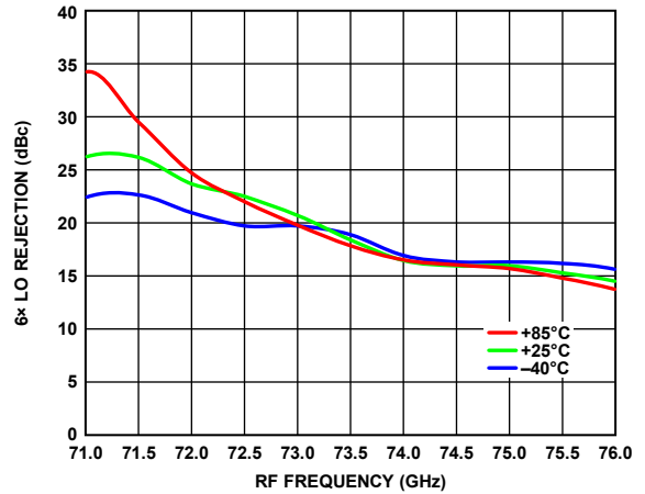
Figure 39. 6\times LO Rejection vs. RF Frequency over Temperature, Gain = 23.5\text{ dB}
