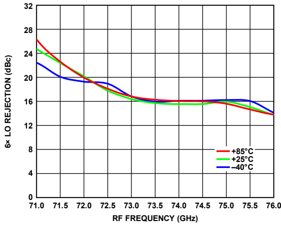
Figure 21. 6x LO Rejection vs. RF Frequency over Temperature, Gain = 23.5 dB
