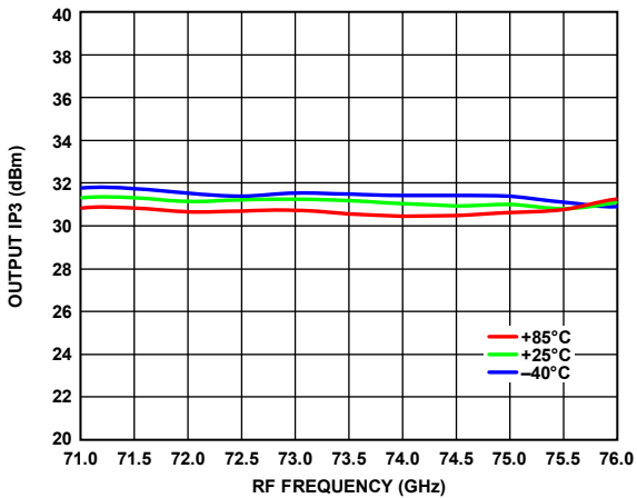
Figure 37. Output IP3 vs. RF Frequency over Temperature, Gain = 23.5\text{ dB}
