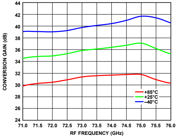
Figure 36. Maximum Conversion Gain vs. RF Frequency over Temperature, IF Input Power = -20\text{ dBm}
