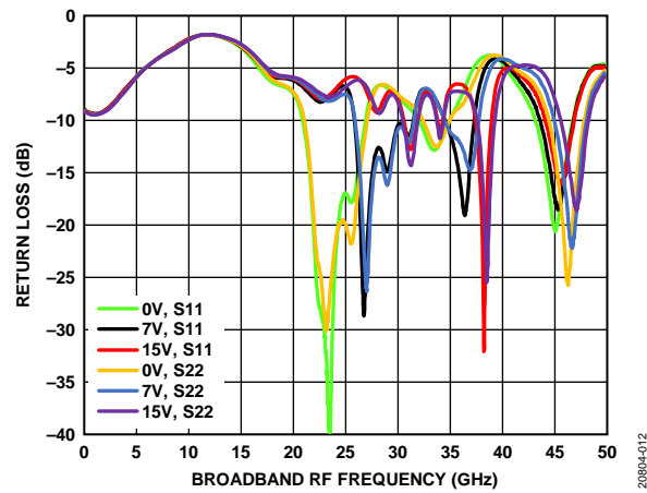
Figure 12. Return Loss vs. Broadband RF Frequency at Various Voltages
