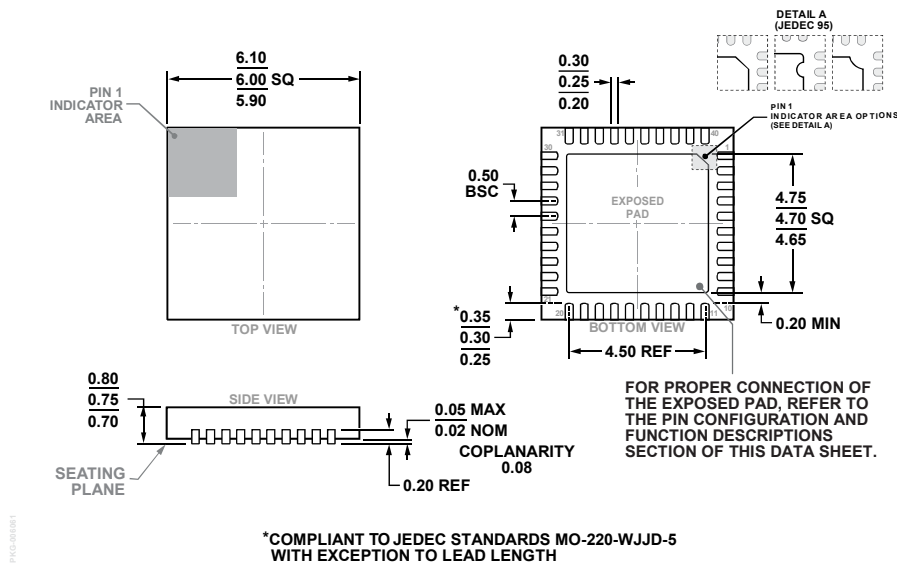
*COMPLIANT TO JEDEC STANDARDS MO-220-WJJD-5 WITH EXCEPTION TO LEAD LENGTH Figure 45. 40-Lead Lead Frame Chip Scale Package [LFCSP] 6 mm × 6 mm Body and 0.75 mm Package Height (CP-40-27) Dimensions shown in millimeters
