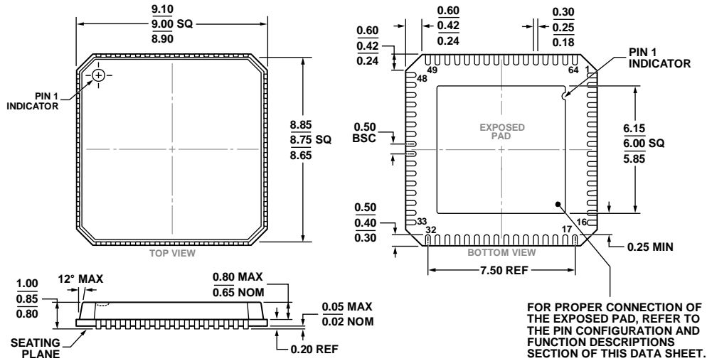
COMPLIANT TO JEDEC STANDARDS MO-220-VMM4 Figure 33. 64-Lead Lead Frame Chip Scale Package [LFCSP_VQ] 9 mm × 9 mm Body, Very Thin Quad (CP-64-2) Dimensions shown in millimeters
