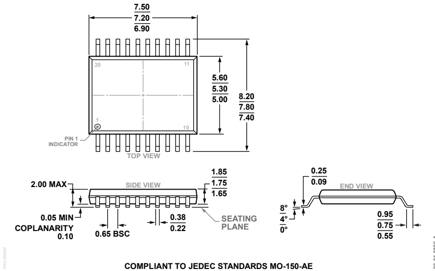
COMPLIANT TO JEDEC STANDARDS MO-150-AE Figure 46. 20-Lead Shrink Small Outline Package [SSOP] (RS-20) Dimensions shown in millimeters
