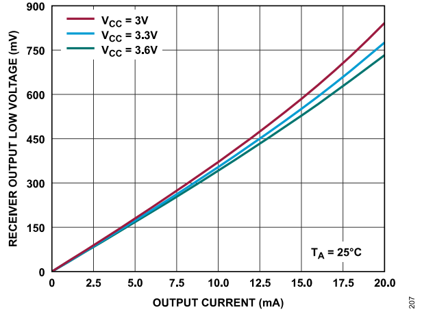
Figure 6. Receiver Output Low Voltage vs. Output Current
