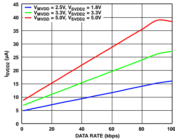
Figure 62. I_{SVDD2} Supply Current vs. Data Rate on All GPIO Channels at Various Supply Voltages, MSS High
