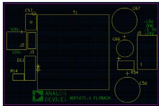
Figure 18. Silkscreen Top
