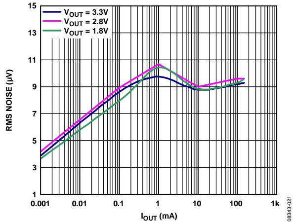
Figure 20. Output RMS Noise vs. Load Current ( I_{OUT} ) and Output Voltage ( V_{OUT} ), V_{IN} = 5V , C_{OUT} = 1µF
