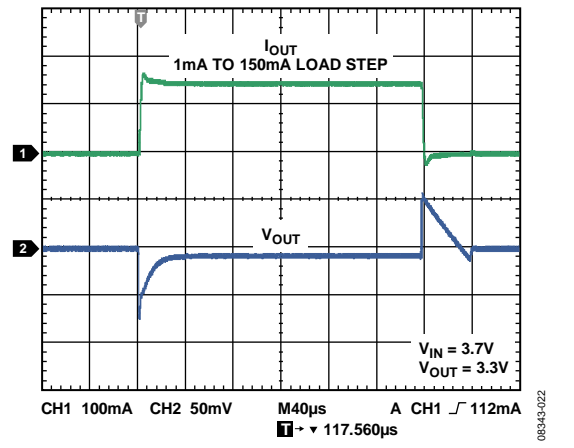
Figure 22. Load Transient Response, C_{OUT} = 1µF
