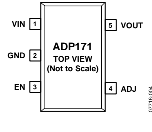
Figure 4. ADP171 5-Lead TSOT
