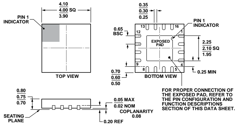
COMPLIANT TO JEDEC STANDARDS MO-220-WGGC. Figure 49. 16-Lead Lead Frame Chip Scale Package [LFCSP_WQ] 4 mm × 4 mm Body, Very Very Thin Quad (CP-16-23) Dimensions shown in millimeters
