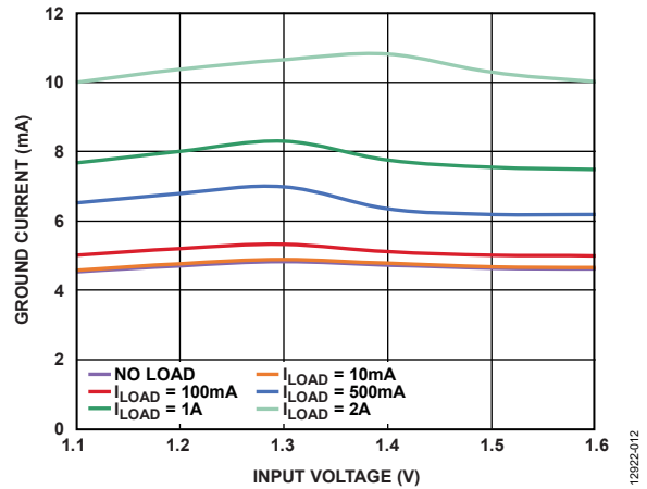
Figure 13. Ground Current vs. Input Voltage (in Dropout), V_{OUT} = 1.3 V
