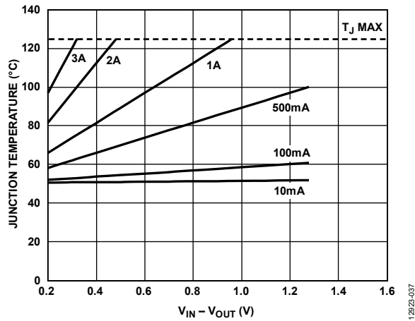
Figure 39. 500 mm 2 of PCB Copper, T A = 50°C
