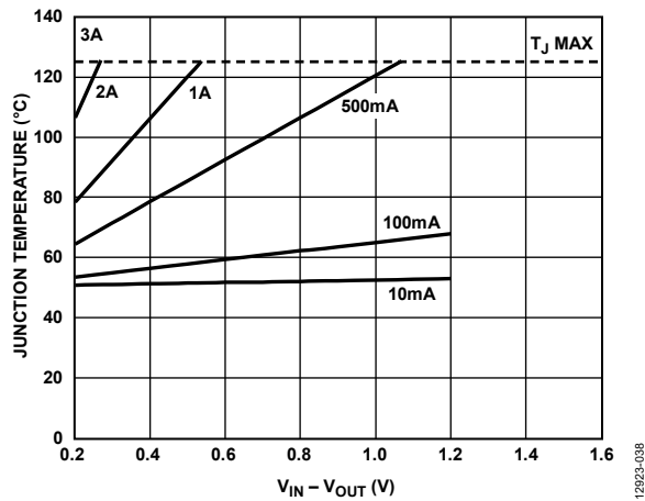
Figure 40. 25 mm 2 of PCB Copper, T A = 50°C
