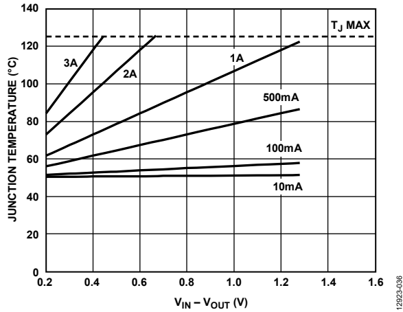
Figure 38. 6400 mm 2 of PCB Copper, T A = 50°C
