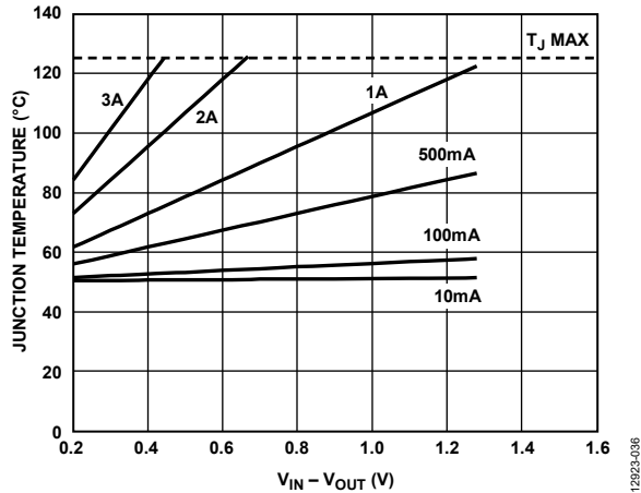
Figure 38. 6400 mm 2 of PCB Copper, T A = 50°C
