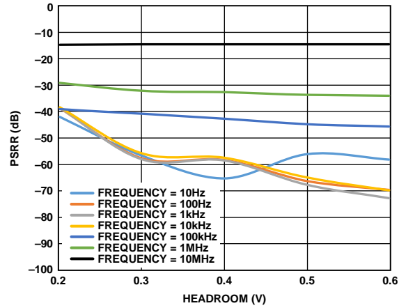
Figure 36. Power Supply Rejection Ratio (PSRR) vs. Headroom Voltage at Various Frequencies, V_{OUT} = 0.9\text{ V} , Load = 5 A
