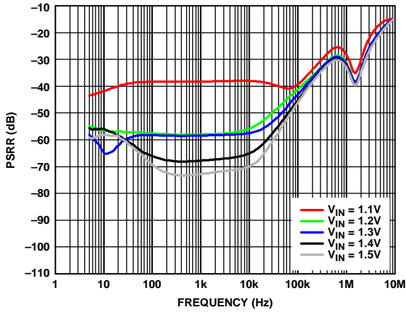
Figure 34. Power Supply Rejection Ratio (PSRR) vs. Frequency at Various Input Voltages ( V_{IN} ), V_{OUT} = 0.9\text{ V} , Load = 5 A
