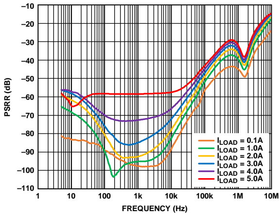
Figure 35. Power Supply Rejection Ratio (PSRR) vs. Frequency at Various Loads ( I_{LOAD} ), V_{OUT} = 0.9\text{ V} , V_{IN} = 1.3\text{ V}
