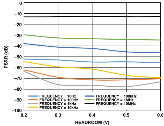
Figure 37. Power Supply Rejection Ratio (PSRR) vs. Headroom Voltage at Various Frequencies, V_{OUT} = 1.3\text{ V} , Load = 5 A
