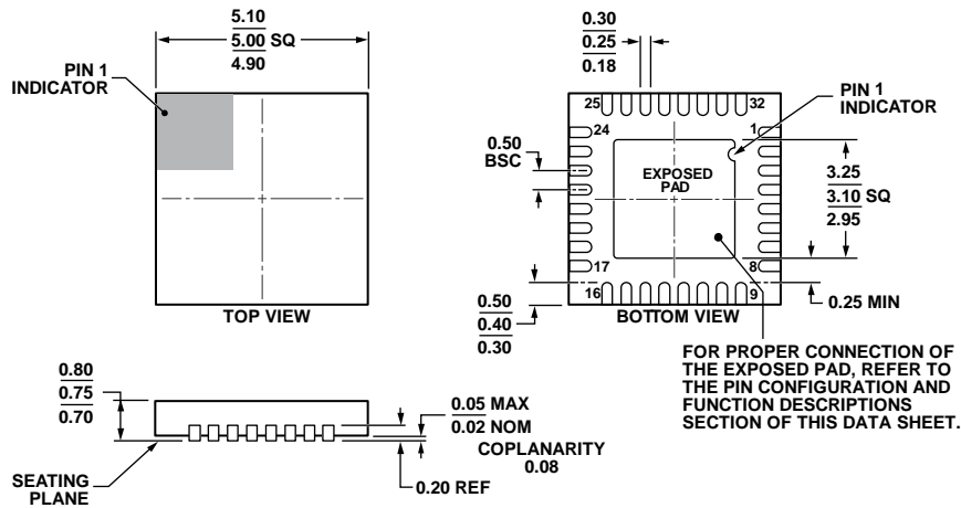
Figure 36. 32-Lead Lead Frame Chip Scale Package [LFCSP] 5 mm x 5 mm Body and 0.75 mm Package Height (CP-32-7)
