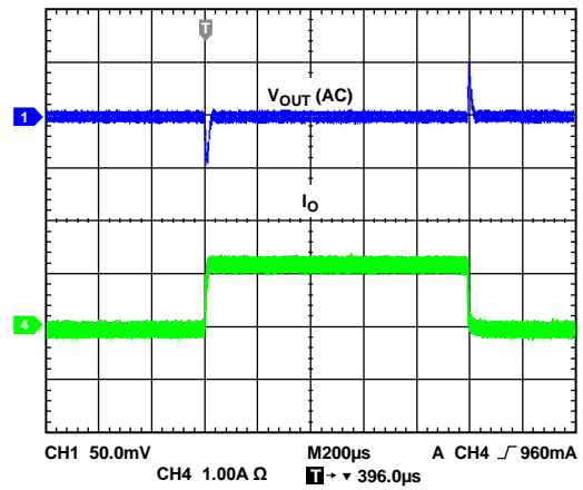
Figure 27. Load Transient (ADP2120, FPWM, V_{IN} = 5V )
