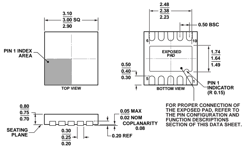
Figure 59. 10-Lead Lead Frame Chip Scale Package [LFCSP_WD] 3 mm x 3 mm Body, Very Very Thin, Dual Lead (CP-10-9) Dimensions shown in millimeters
