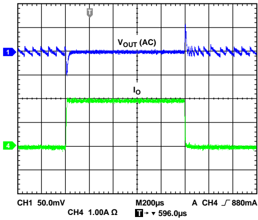
Figure 23. Load Transient (ADP2119, PFM, V_{IN} = 5V )
