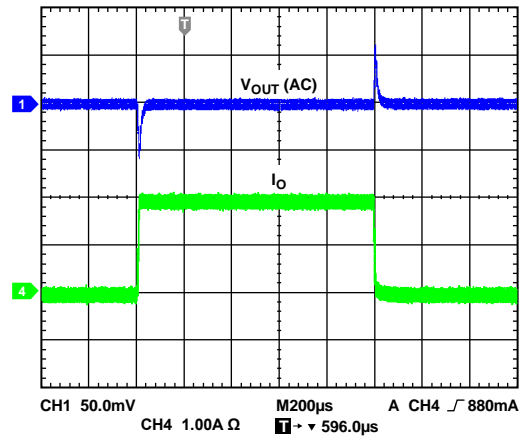
Figure 26. Load Transient (ADP2119, FPWM, V_{IN} = 5V )
