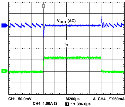
Figure 24. Load Transient (ADP2120, PFM, V_{IN} = 5V )
