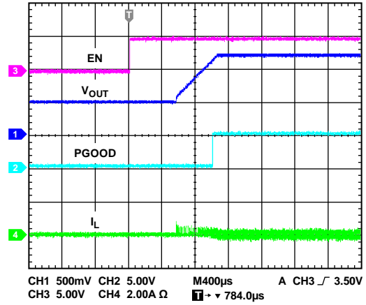
Figure 25. Soft Start with Precharged Output (ADP2119, V_{IN} = 5V )
