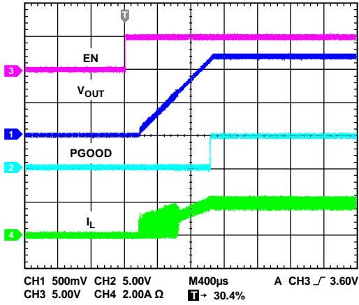
Figure 22. Soft Start with Full Load (ADP2119, V_{IN} = 5V )
