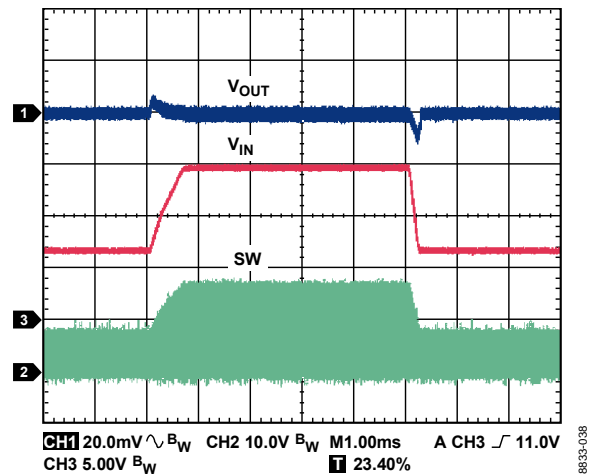
Figure 38. ADP2302 Line Transient, 7\text{ V} to 15\text{ V} , V_{OUT} = 3.3\text{ V} , I_{OUT} = 2\text{ A} , L = 6.8\ \mu\text{H} , C_{OUT} = 2 \times 22\ \mu\text{F}
