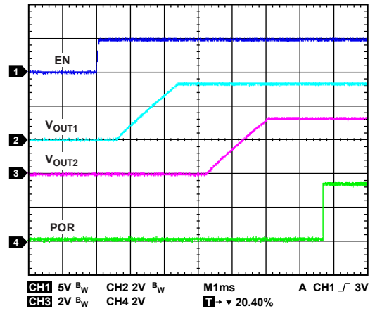
Figure 27. Soft Start with Full Load
