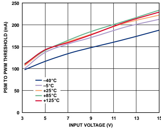
Figure 60. PSM to PWM Mode Transition vs. Input Voltage, Different Temperatures
