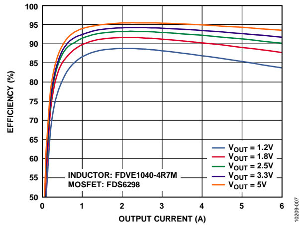
Figure 7. Efficiency at V_{IN} = 12\text{ V} , f_{SW} = 250\ \text{kHz}
