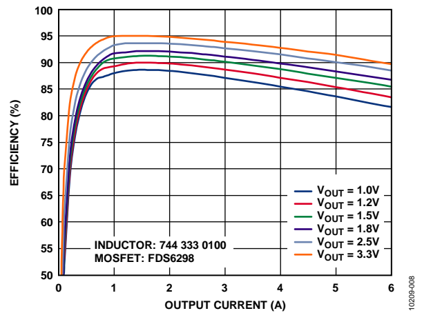
Figure 8. Efficiency at V_{IN} = 5\text{ V} , f_{SW} = 500\ \text{kHz}
