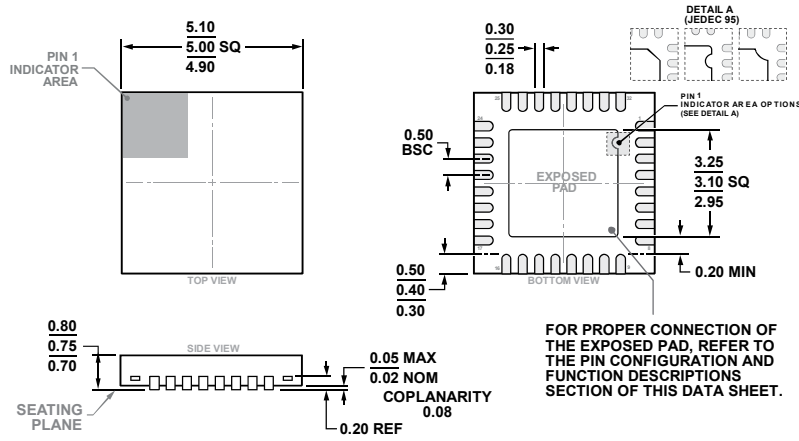
Figure 76. 32-Lead Lead Frame Chip Scale Package [LFCSPP] 5 mm × 5 mm Body and 0.75 mm Package Height (CP-32-7)
