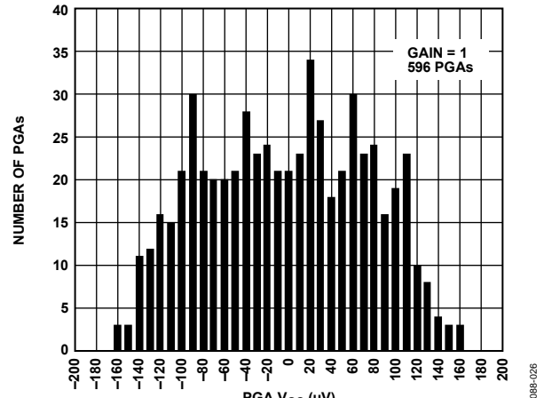
Figure 27. PGA Input Offset Voltage Distribution
