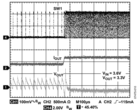
Figure 20. Mode Change by Load Transients, Load Rise ( V_{IN} = 3.6V , V_{OUT} = 3.3V )
