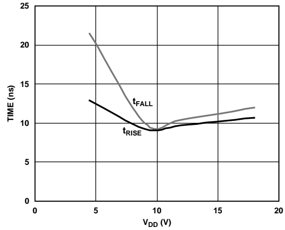
Figure 8. Rise and Fall Times vs. V_{DD}
